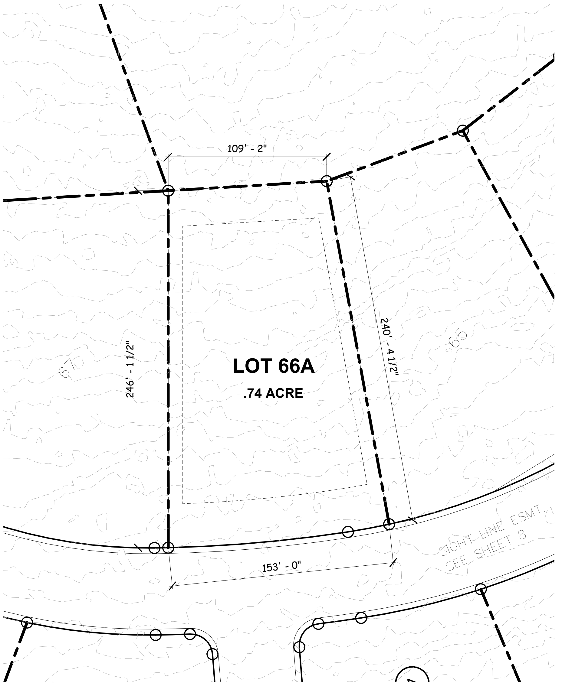
① SITE PLAN - LOT 66A 1" = 40'-0"
