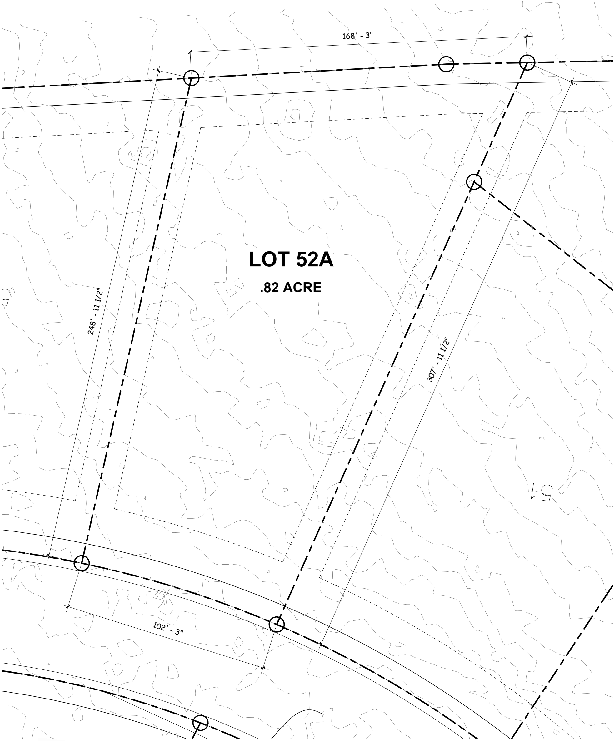
① SITE PLAN- LOT 52A 1" = 30'-0"
