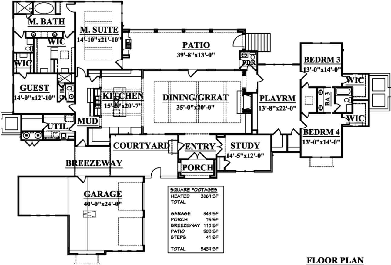
FLOOR PLAN 14036 ©2015 EPPRIGHT HOMES L.L.C.
