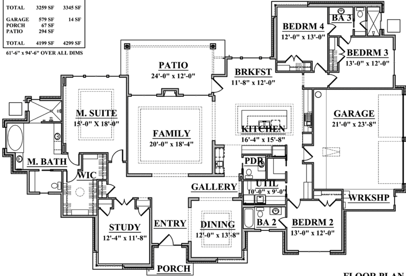
FLOOR PLAN 12002
