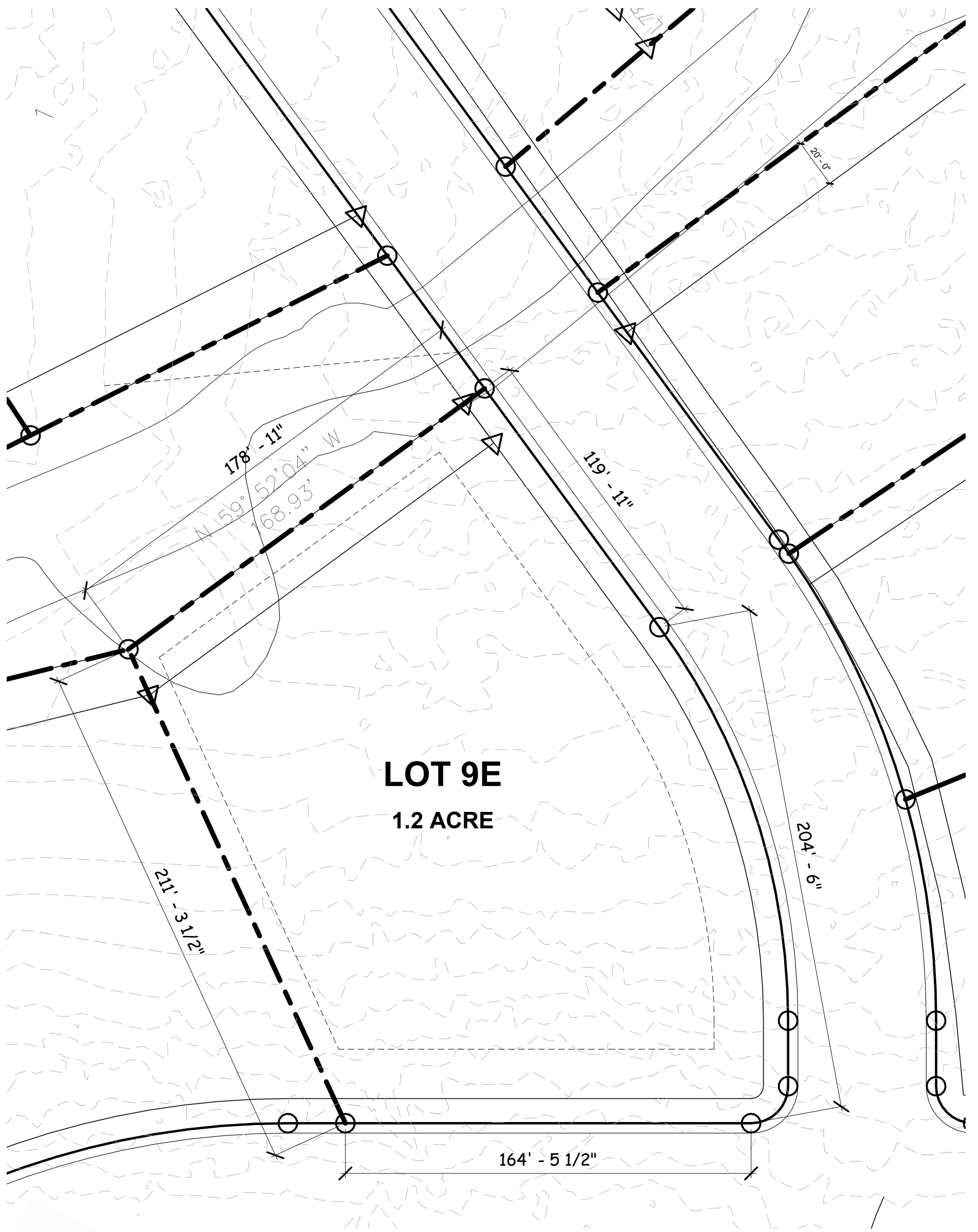
① SITE PLAN - LOT 9E 1" = 40'-0"
