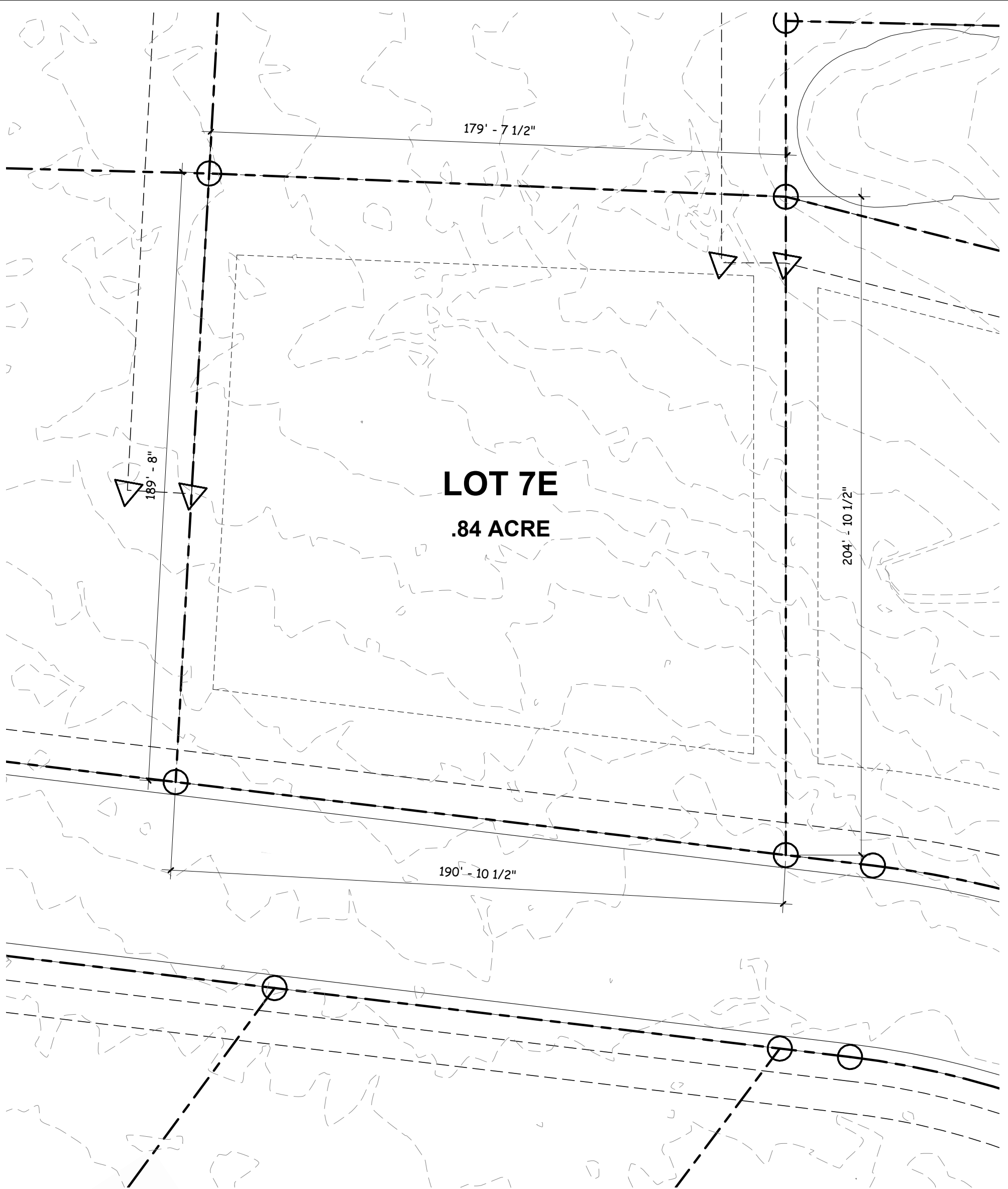
① SITE PLAN- LOT 7E 1" = 30'-0"
