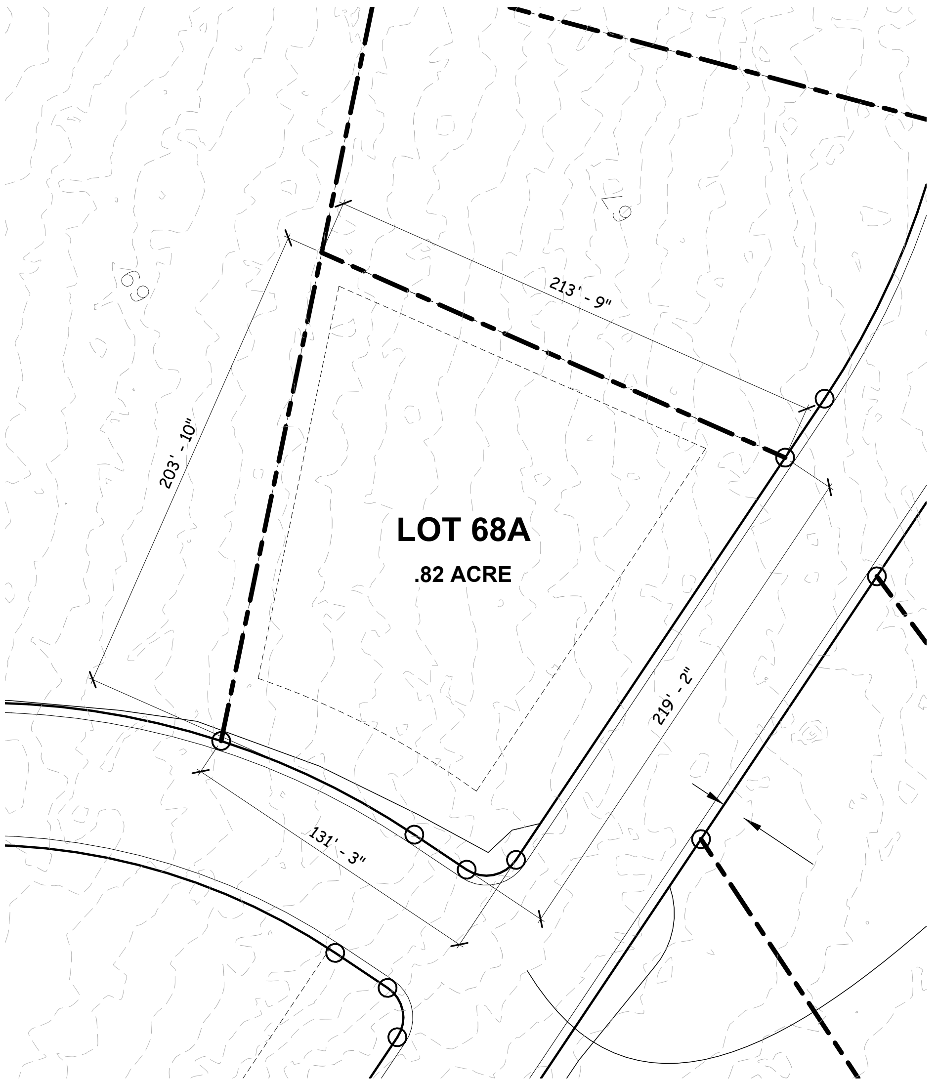
① SITE PLAN - LOT 68A 1" = 40'-0"
