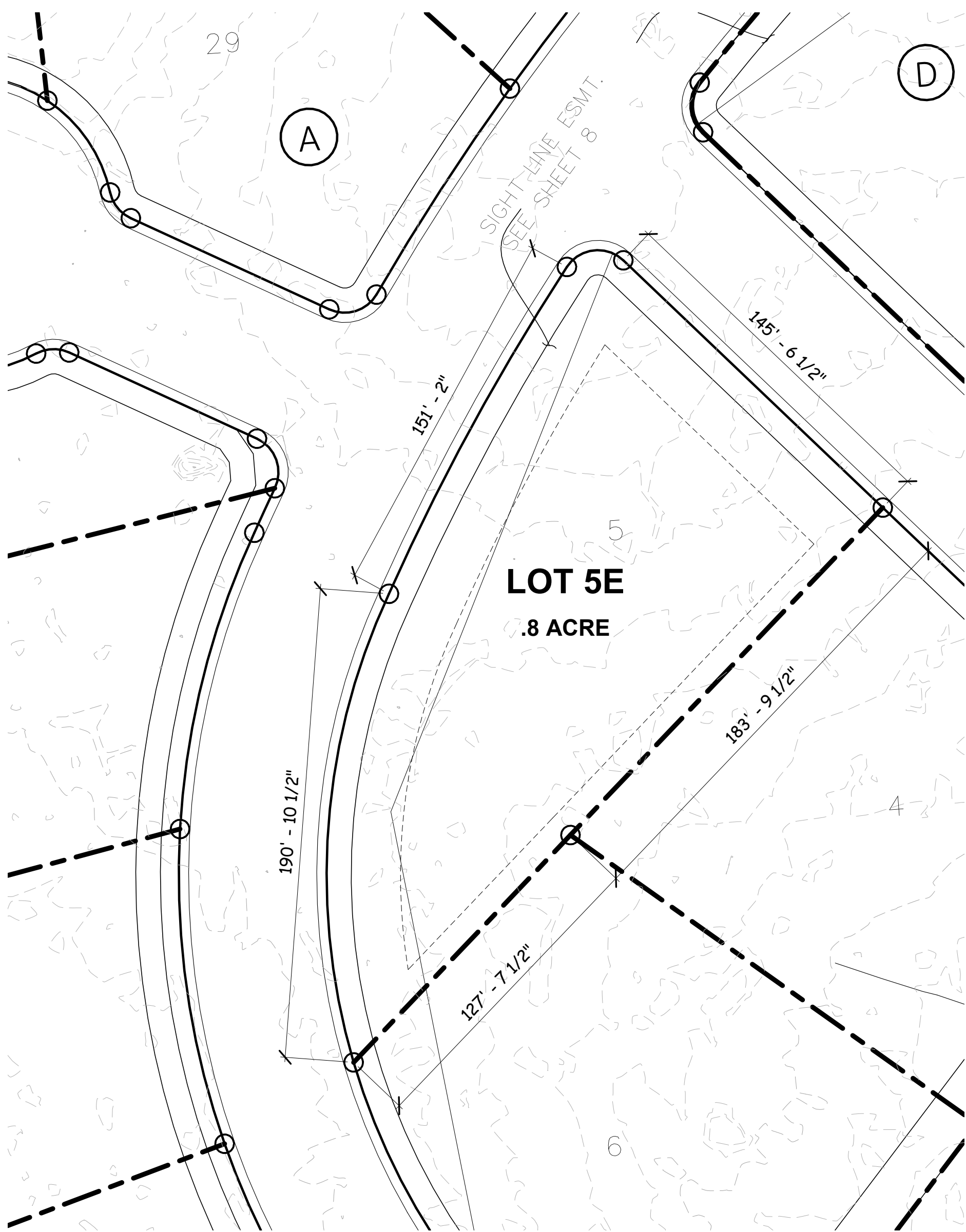
① SITE PLAN - LOT 5E 1" = 40'-0"
