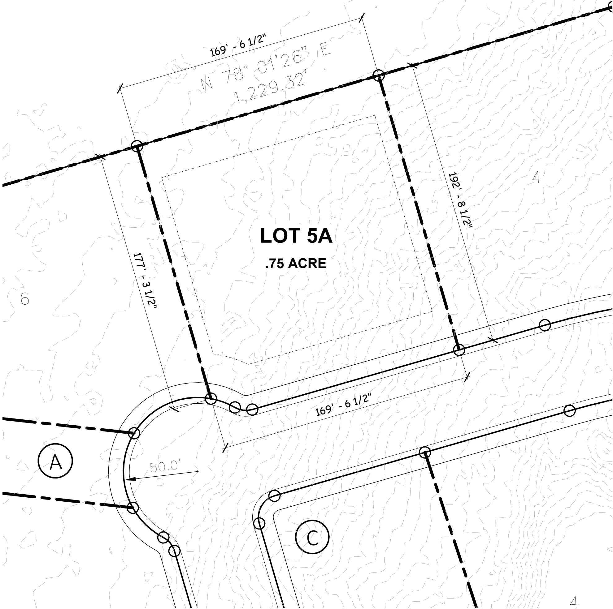
① SITE PLAN - LOT 5A 1" = 40'-0"
