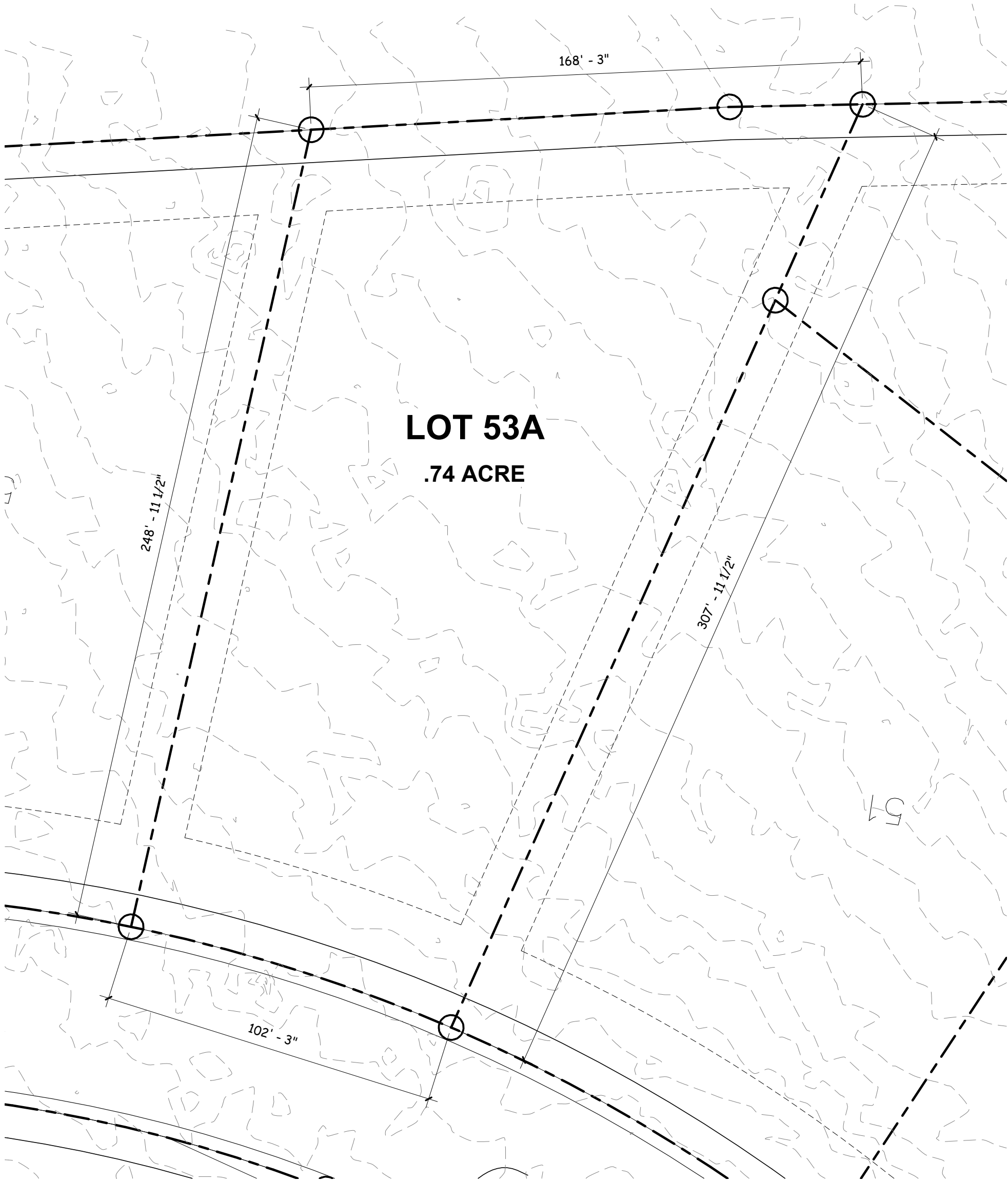
① SITE PLAN- LOT 53A 1" = 30'-0"
