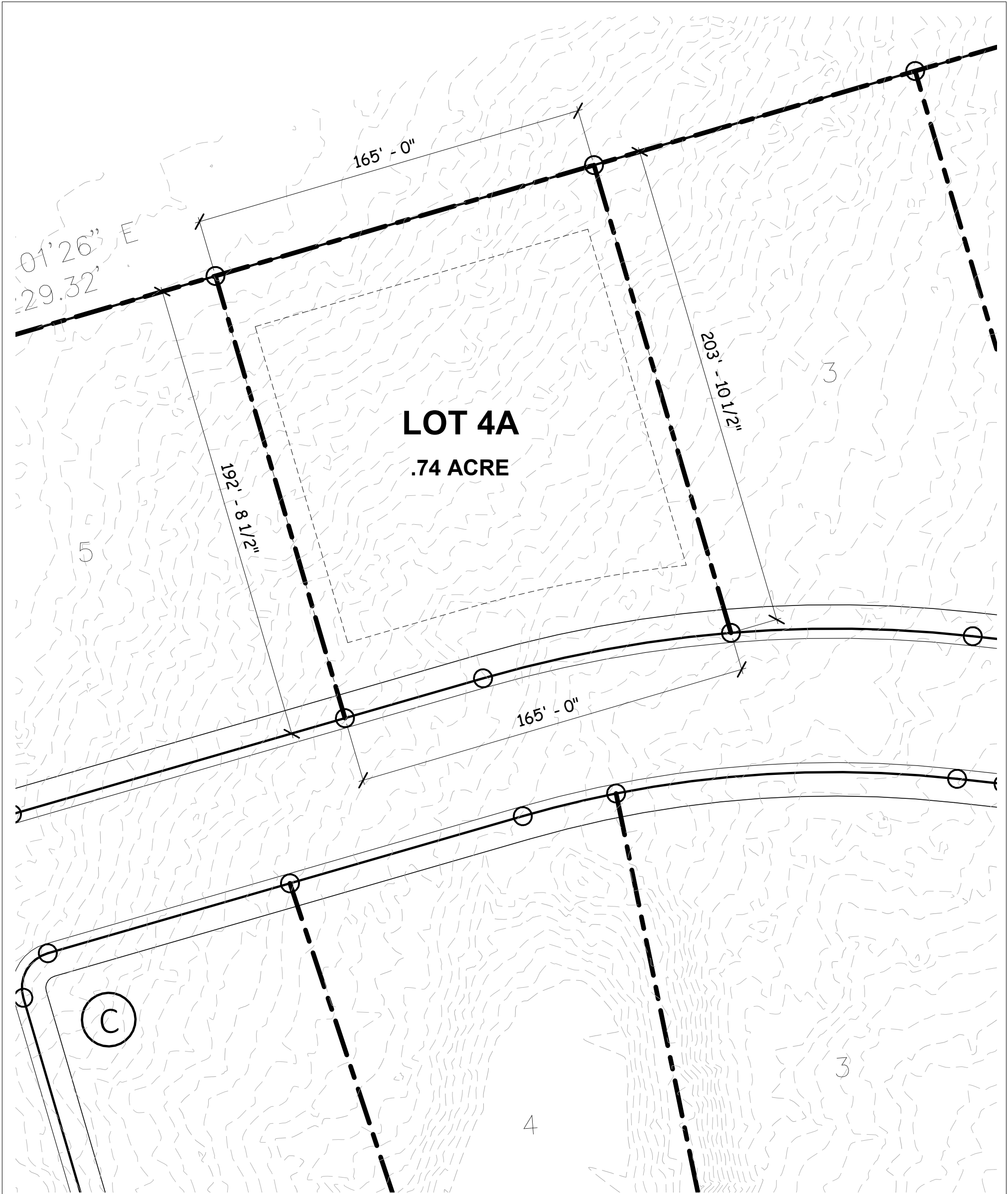
① SITE PLAN - LOT 4A 1" = 40'-0"
