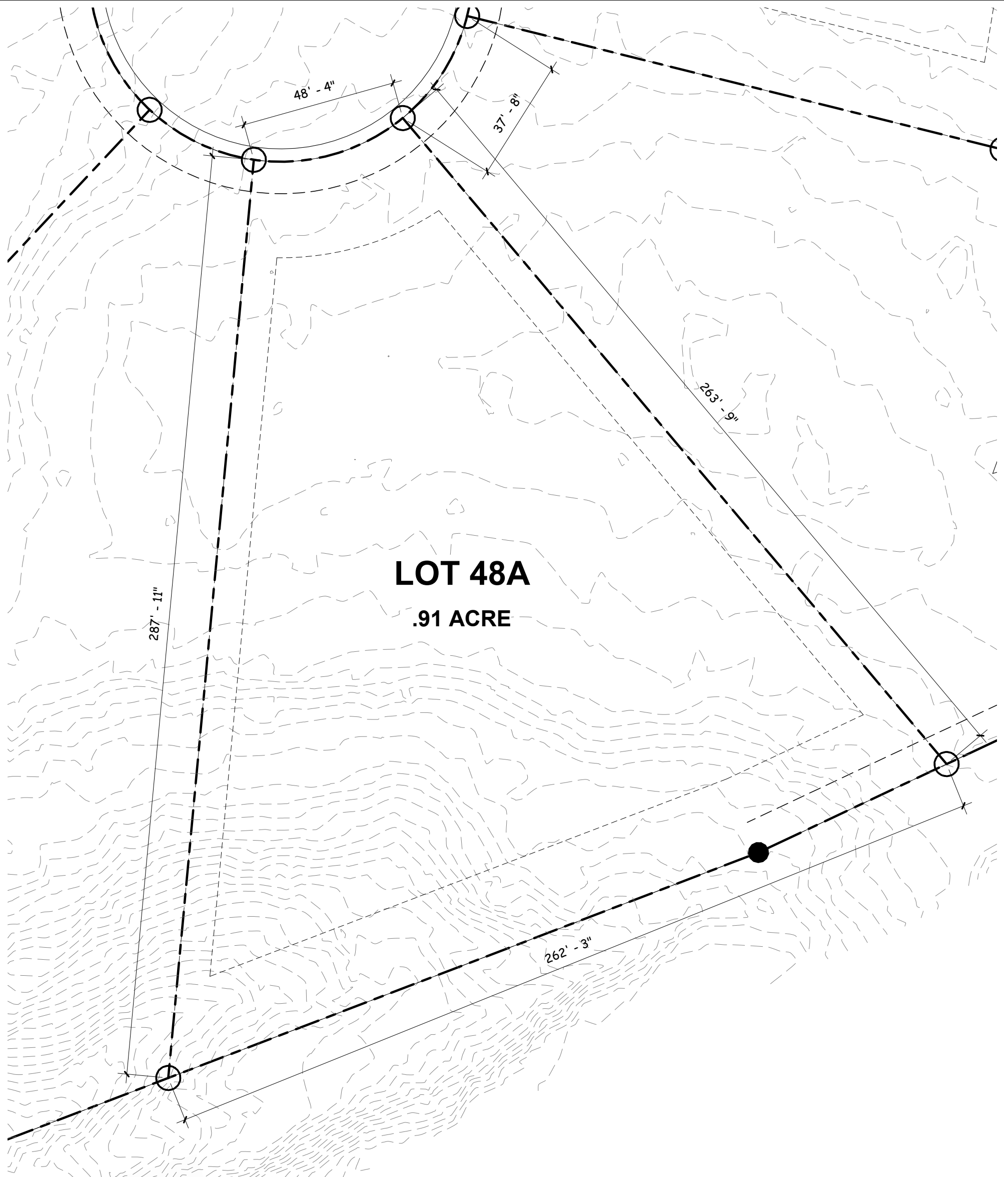
① SITE PLAN- LOT 48A 1" = 30'-0"
