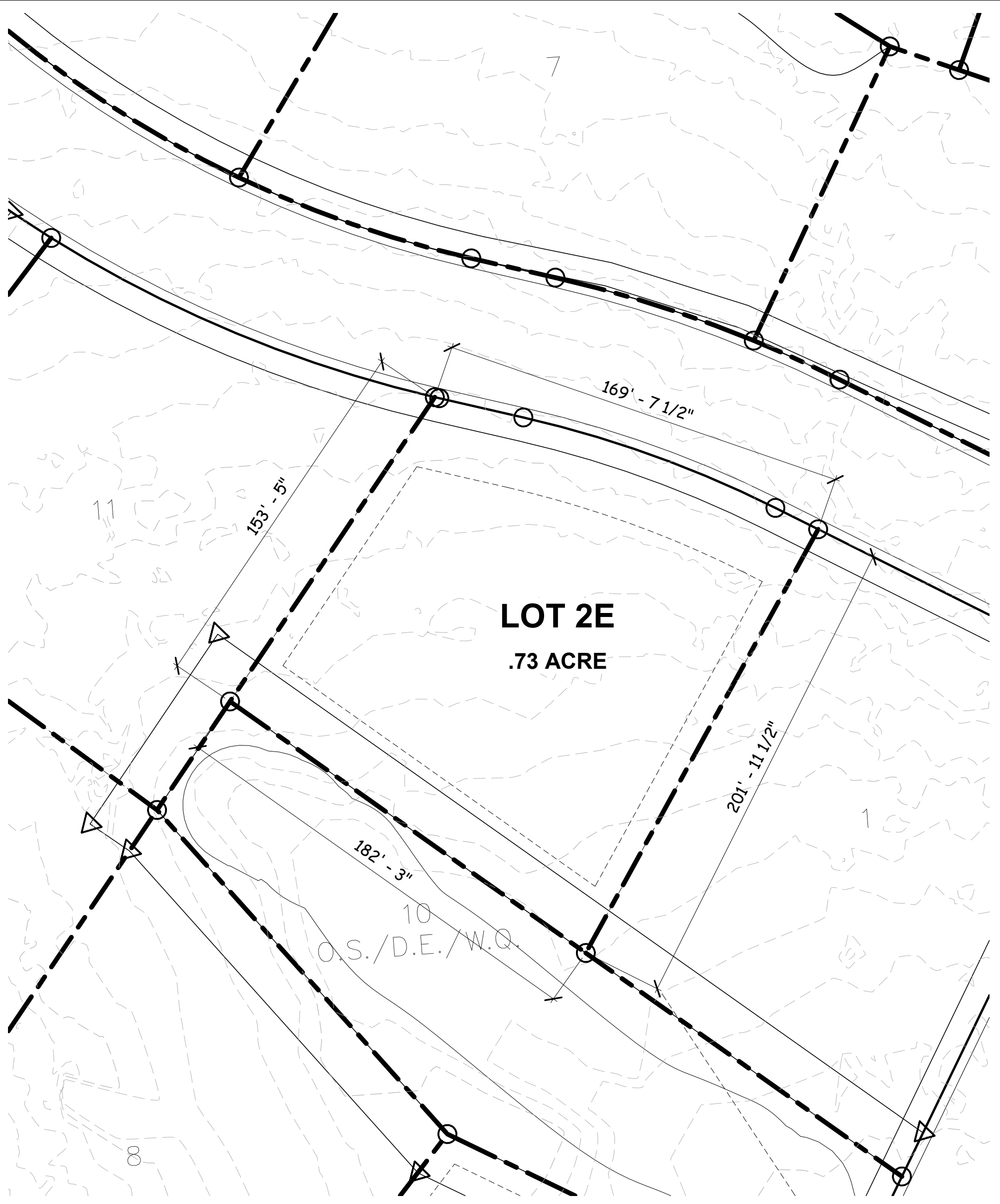
① SITE PLAN - LOT 2E 1" = 40'-0"
