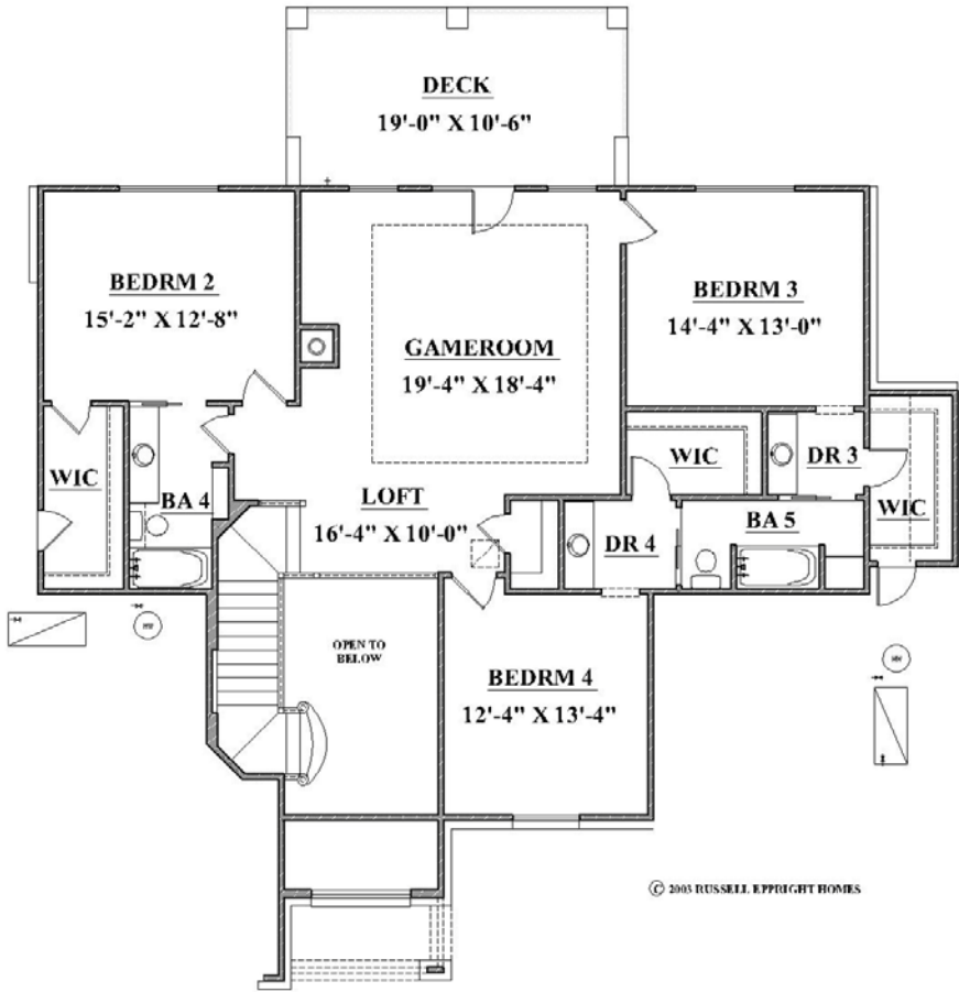
UPPER FLOOR PLAN 98001-P
