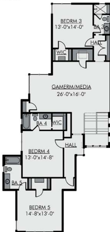
UPPER FLOOR PLAN 506 BOWCROSS POINT ©2016 EPPRIGHT HOMES L.L.C.
