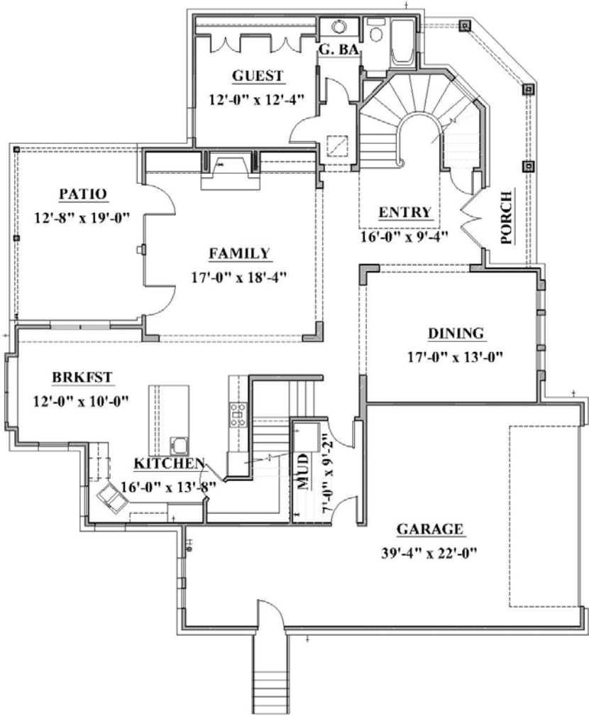
LOWER FLOOR PLAN 00026-P
